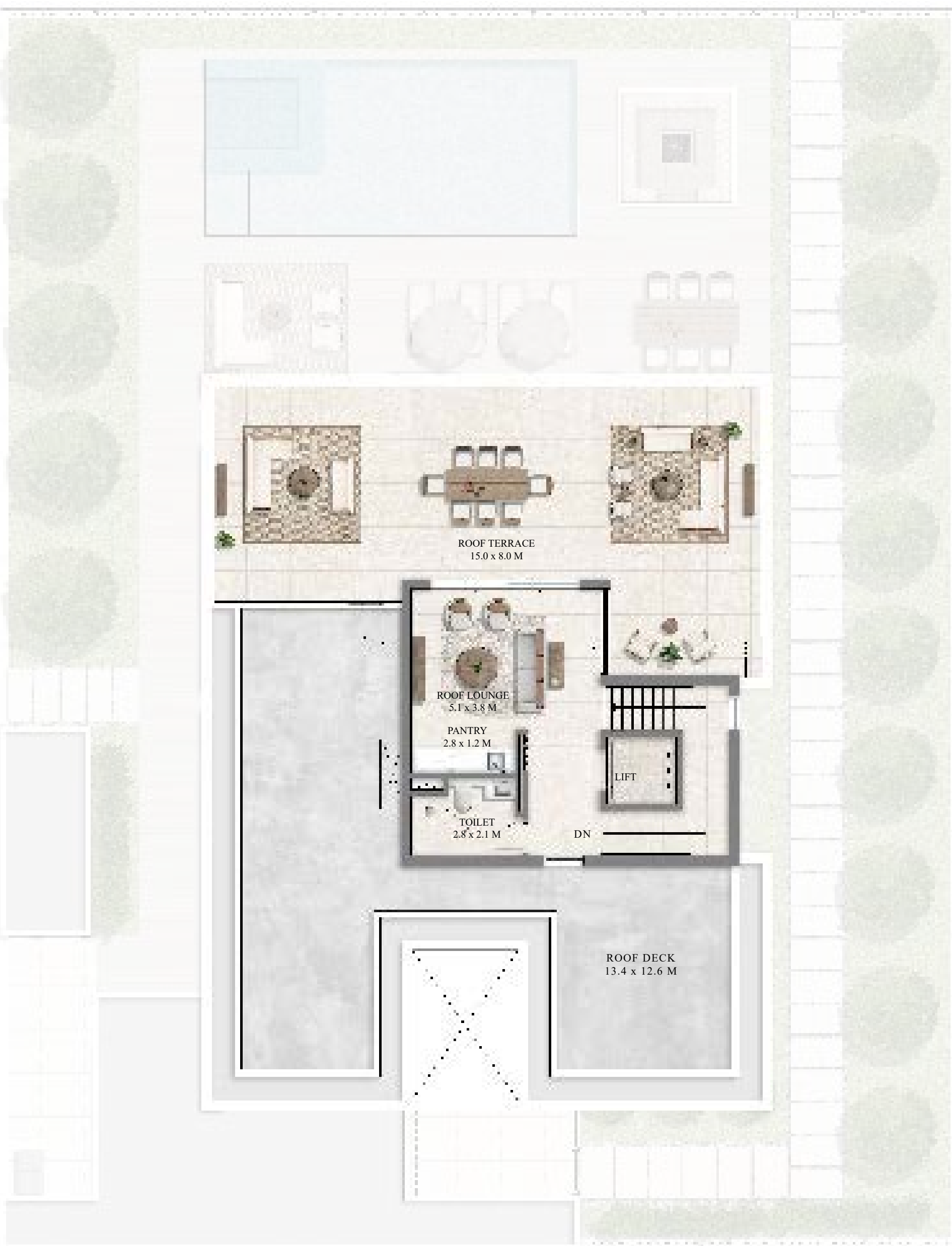
SECOND FLOOR
